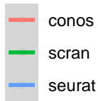
method
