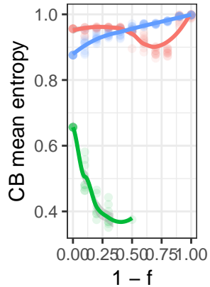
CB entropy
