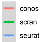
method
