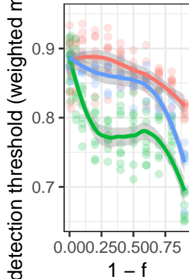
detection
