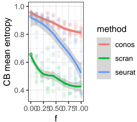
CB entropy
