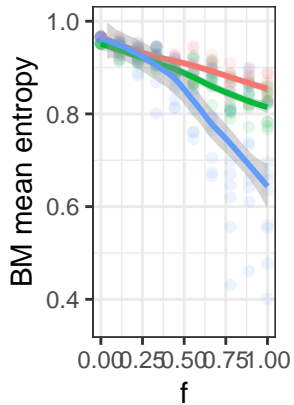
BM entropy
