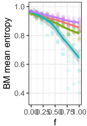
BM entropy
