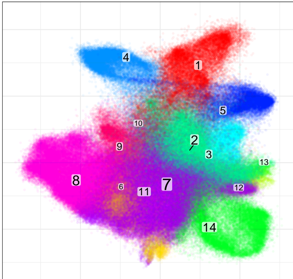
multilevel
