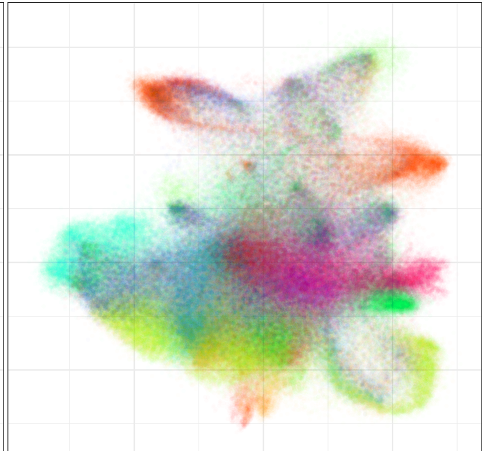
batch
