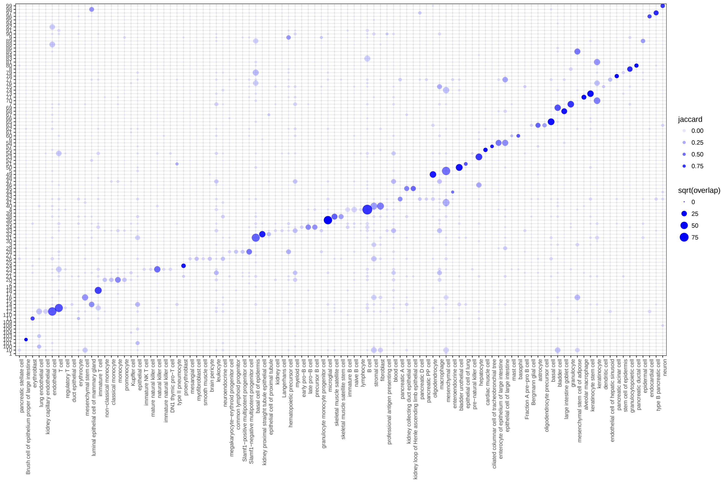
multilevel clusters
