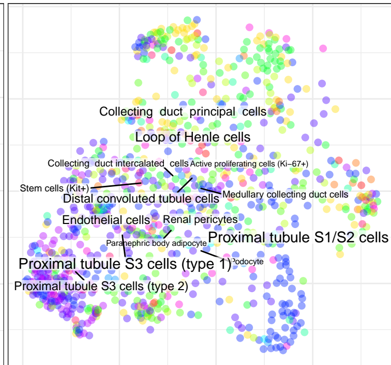
annotation: ATAC
