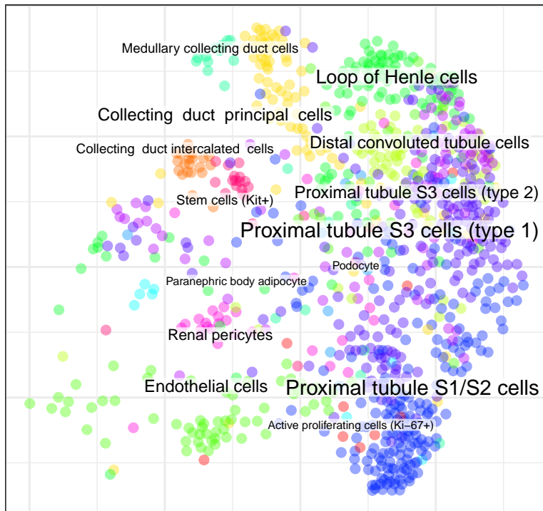
annotation: RNA
