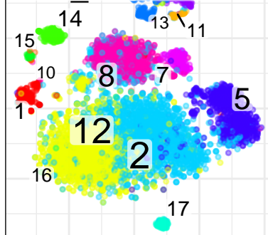
BC7_TUMOR
