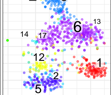
BC6_TUMOR
