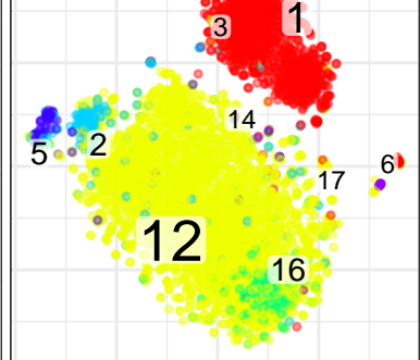
BC3_TUMOR
