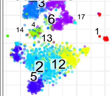
BC8_TUMOR
