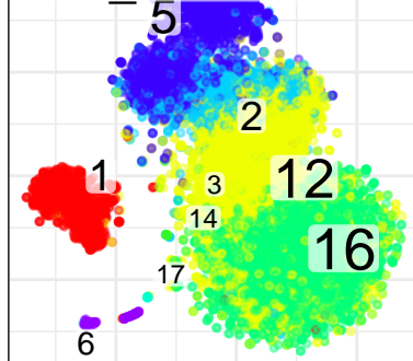
BC7_NORMAL
