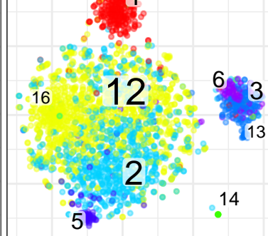
BC3_NORMAL
