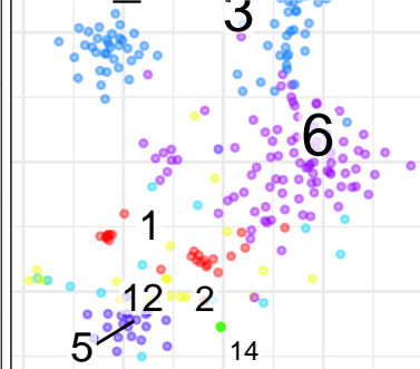
BC5_TUMOR
