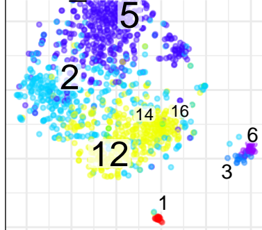
BC4_BLOOD
