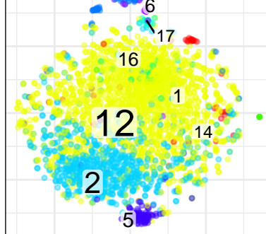
BC2_TUMOR
