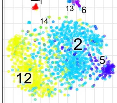
BC4_TUMOR
