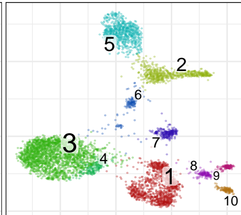
Clusters
