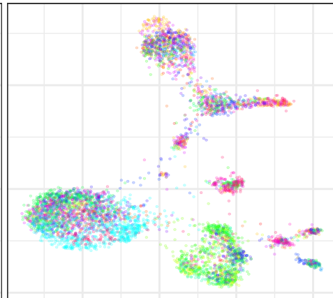
Samples
