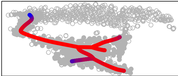
cluster 9
