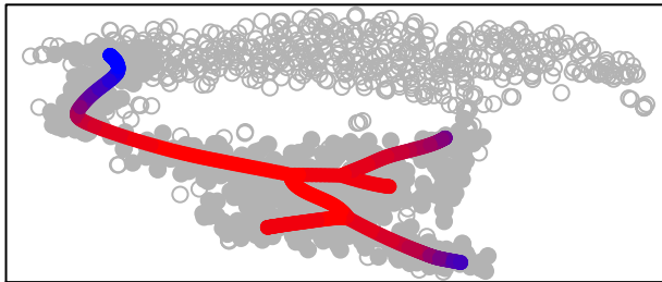
cluster 21
