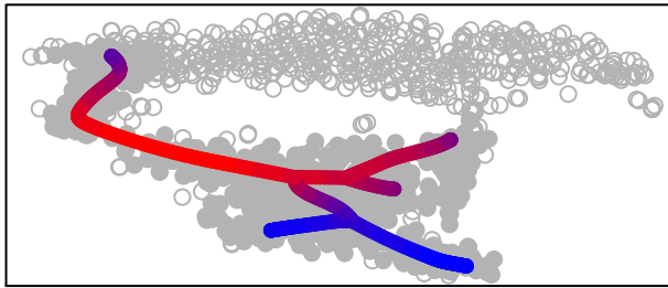
cluster 2
