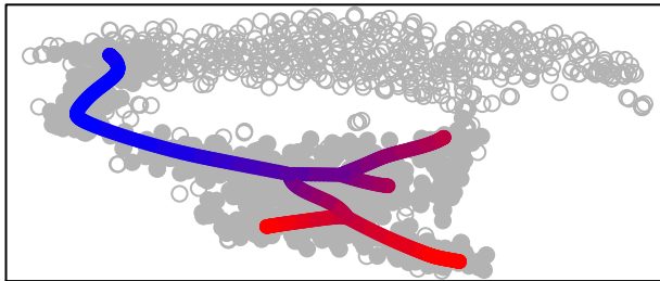
cluster 7
