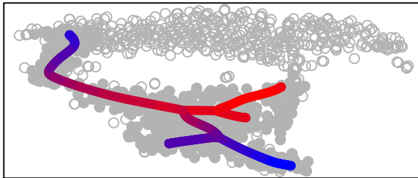
cluster 1
