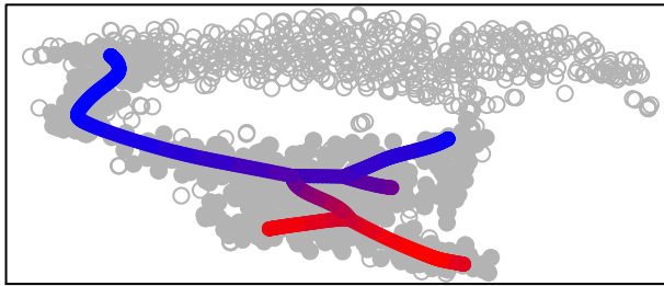
cluster 14
