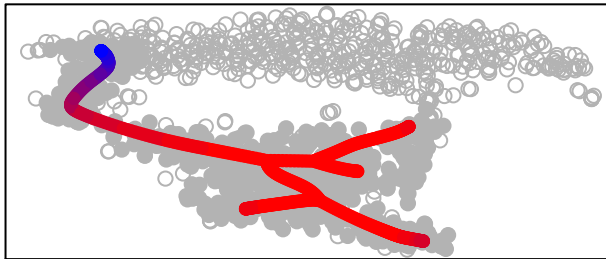
cluster 4
