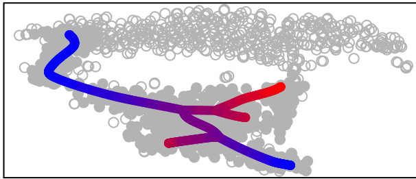
cluster 8
