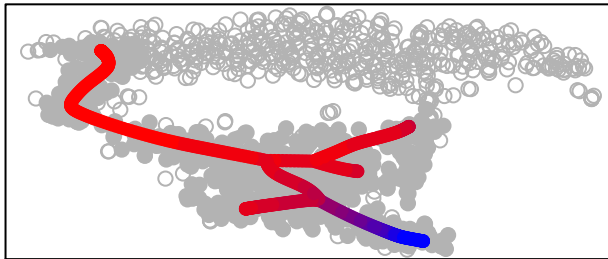
cluster 11
