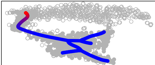
cluster 5
