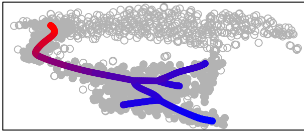
cluster 16
