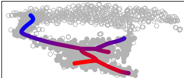
cluster 15
