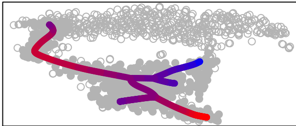
cluster 20
