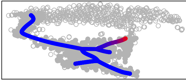
cluster 18
