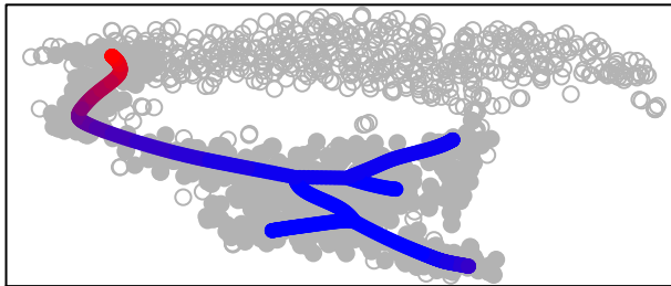
cluster 12
