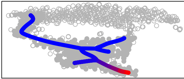
cluster 3
