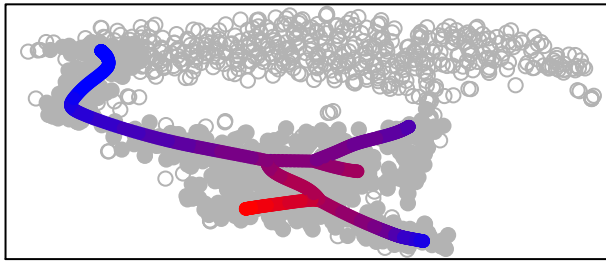
cluster 17
