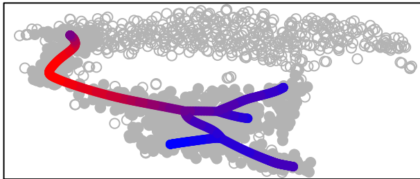
cluster 10
