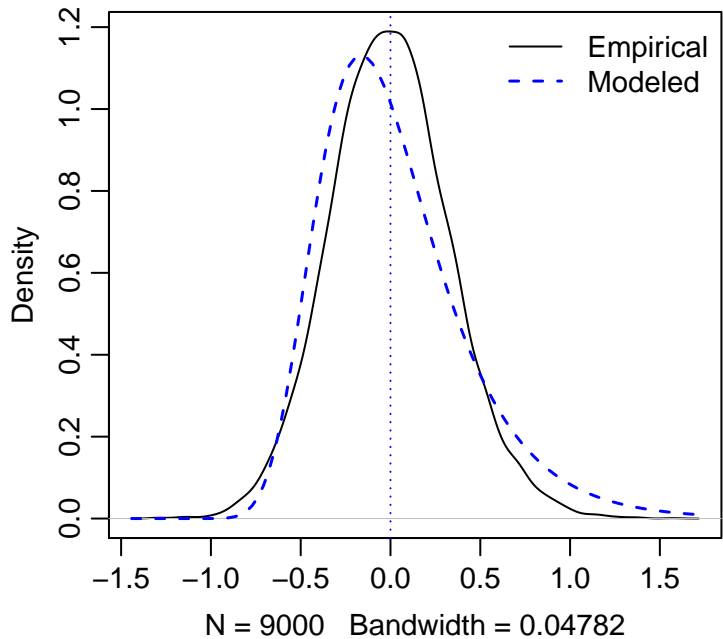
Gumbel fit
