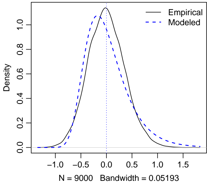
Gumbel fit
